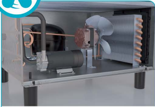
HAVA SOĞUTMALI SİSTEM AIR COOLED SYSTEM
